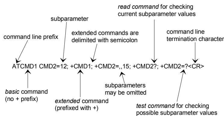
Figure 4: Basic structure of a command line
