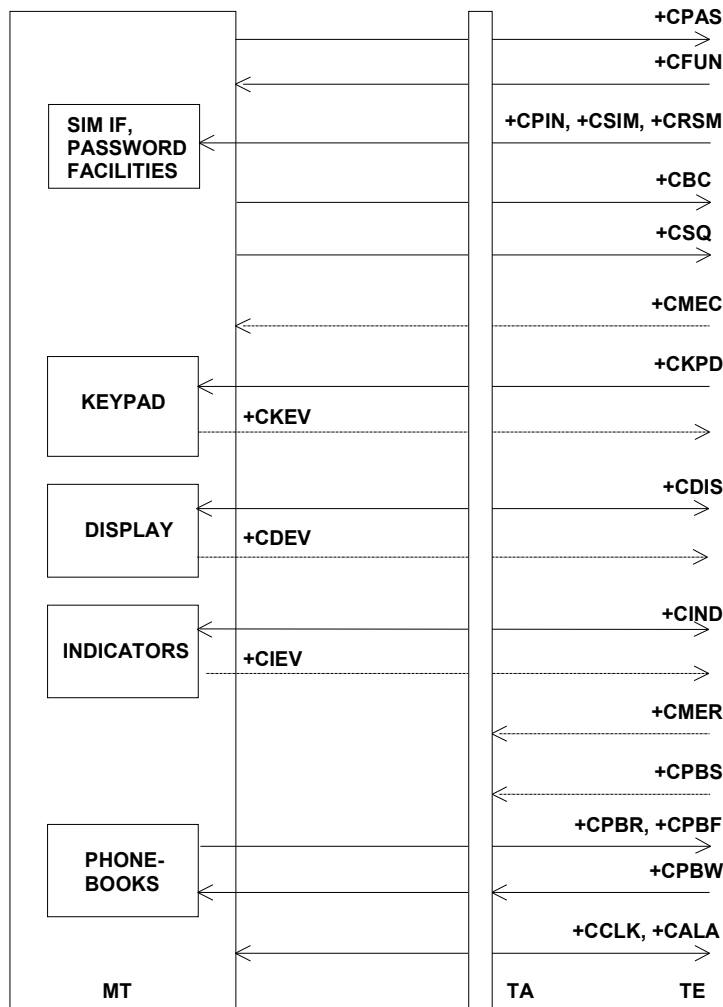
Figure 14: Mobile termination control and status commands
