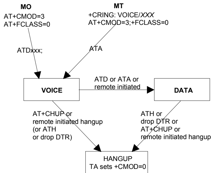
Figure 9: Voice followed by data call
