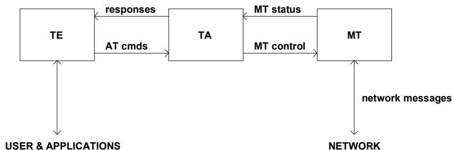
Figure 2: Setup
