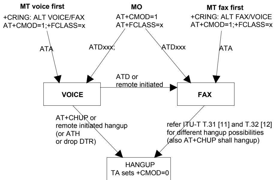
Figure 13: Alternating voice and fax call
