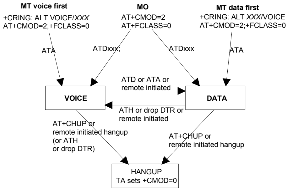
Figure 11: Alternating voice and data call
