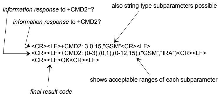
Figure 7: Response to a command line
