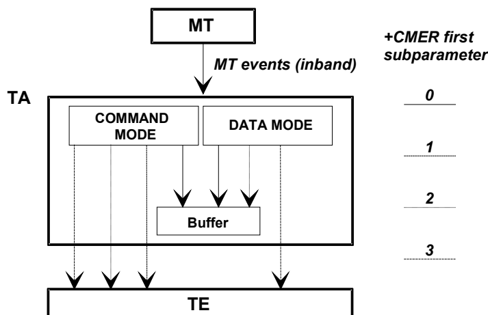
Figure 16: Mobile termination event reporting
